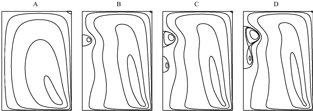
FIGURE 1. Typical representatives of the four topologies (iso-curves of the stream function \psi ) we observe in the present study, here for \gamma = 0.012 and h = 2.2 . Only the right-hand half of the meridional plane is shown. The vertical line to the left is the cylinder axis. A: Re = 700 , no bubbles. B: Re = 1680 , one bubble. C: Re = 1800 , two bubbles. D: Re = 2080 , one bubble with inner structure.
