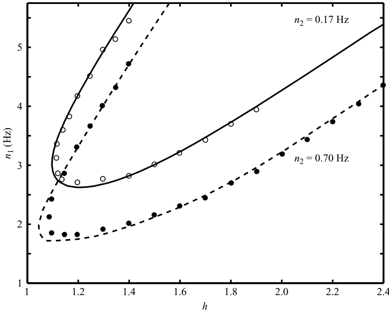
FIGURE 9. Computational bifurcation diagram for non-zero rotation ratios compared with experiments (open and closed circles) by Bar-Yoseph et al. (1990a). Below the curves there are no bubbles, above the curves a single bubble exists.
